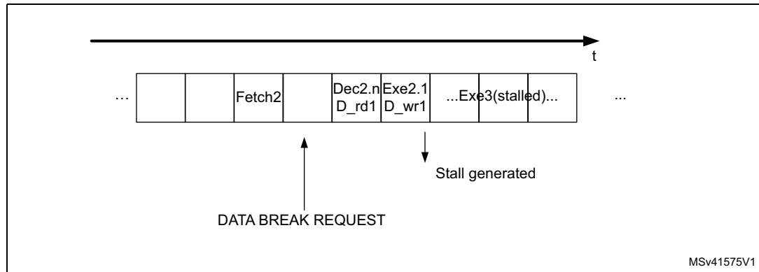
Figure 14. STM8 DM data breaktiming
