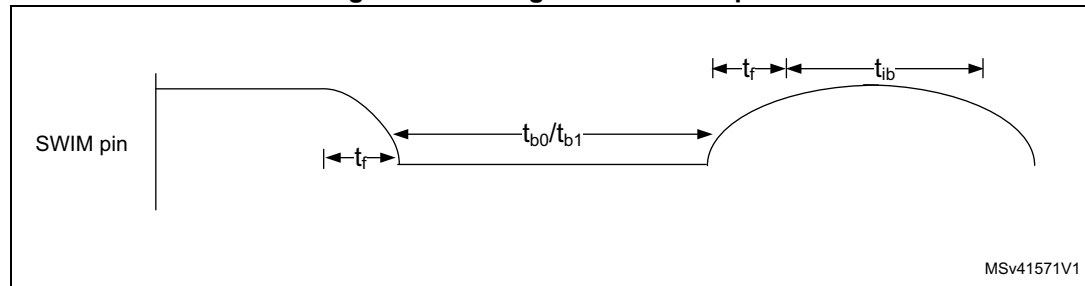
Figure 10. Timings on the SWIM pin
